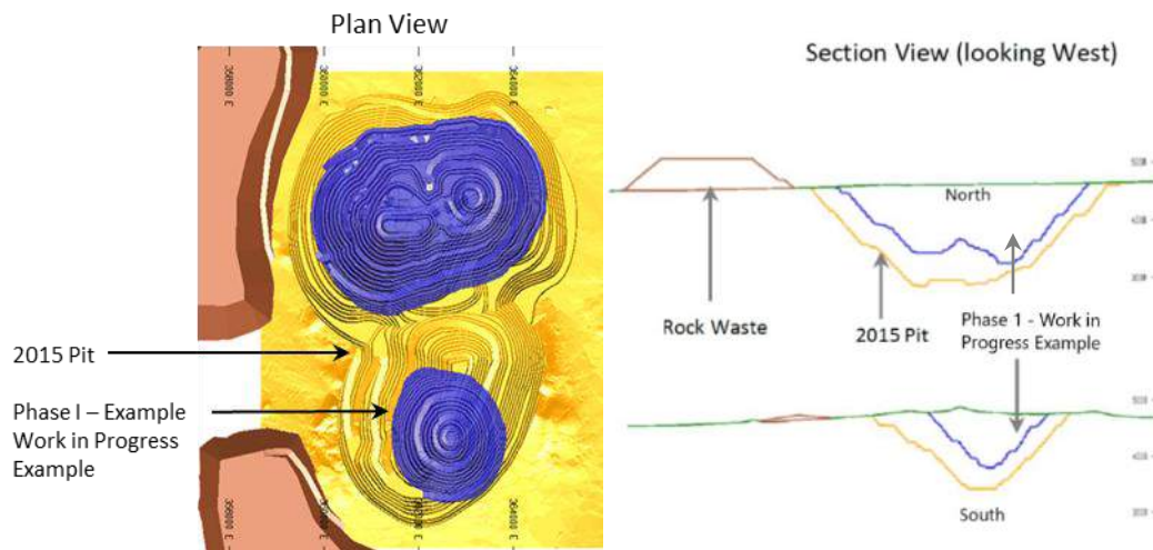
Figure 3 – Work in Progress Example Potential Phase 1 Open Pit Processing Plant Design
